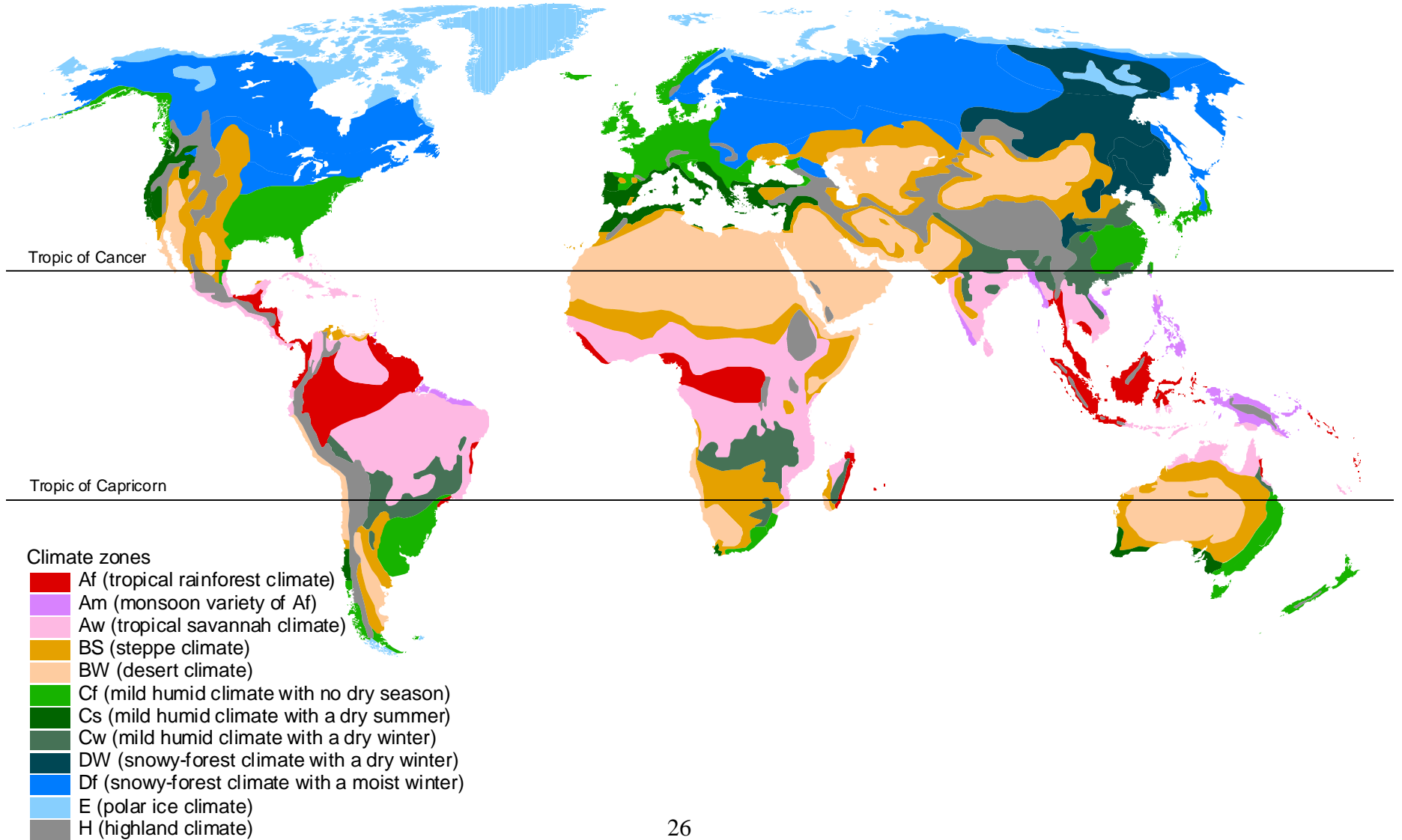
Figure 1. Koppen-Geiger climate zones
